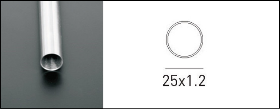
QT - 110 Stainless Steel tube AISI 304, Diameter 25mm, Thickness 1,2mm.
