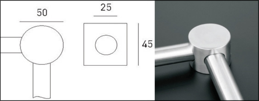
QT - 132 Tube connector at 90° made in Stainless Steel AISI 304.
