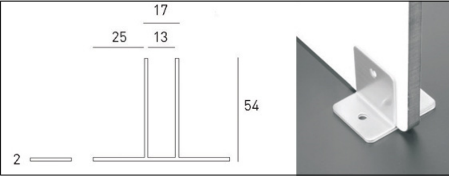
QT - 134 Panel support made in Stainless Steel AISI 304.
