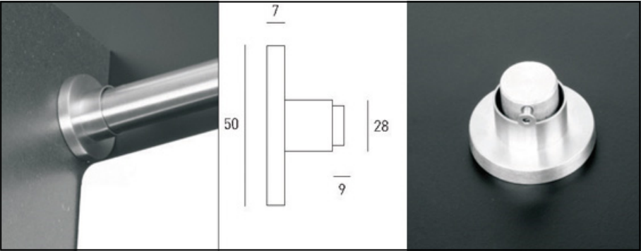
QT - 111 Tube support wall mounting made in Stainless Steel AISI 316 (rose cover) and AISI 304 and brass.
