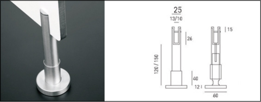
QT - 117 Adjustable foot made in Stainless Steel AISI 316 (rose cover) and AISI 304. Fixing on the floor trough a strong Aluminum base. The height is adjustable even with the base already fixed on the floor and the panel on the support.
