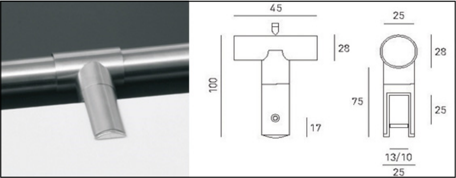
QT - 112 Upper panel holder made in Stainless Steel rotative.
