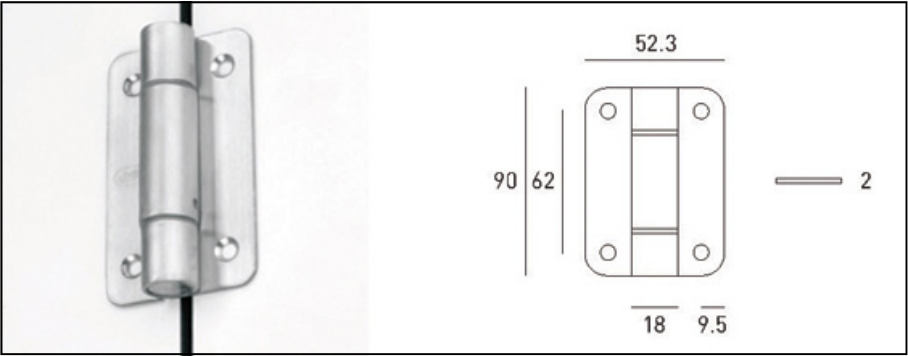
QT - 105 - C Stainless Steel hinge AISI 304 with spring.
