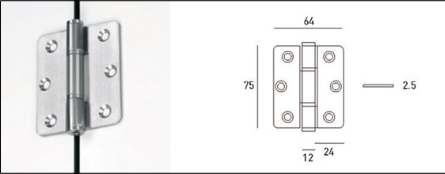
QT - 105 - D Stainless Steel hinge AISI 304.
