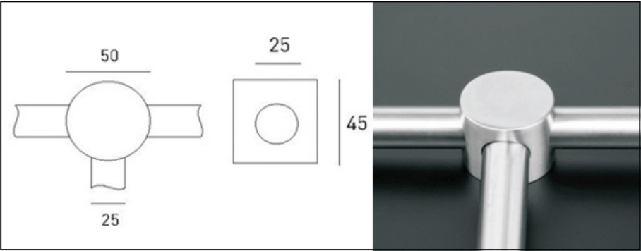
QT - 133 Tube connector at 90° and 180° made in Stainless Steel AISI 304.
