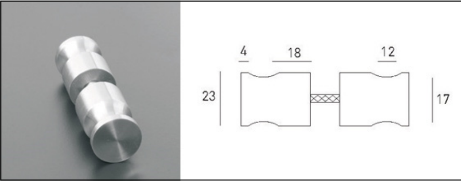
QT - 120 Back to back door knob, anti-vandalism fixing, made in Stainless Steel AISI 304.
