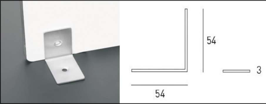
QT - 144 Panel support made in Stainless Steel AISI 304.
