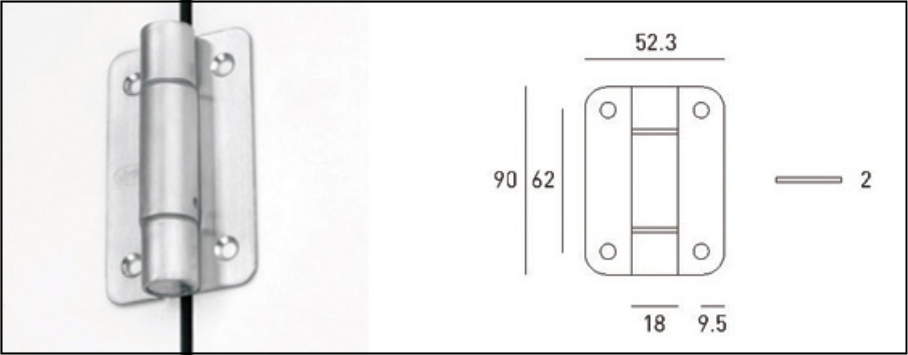
QT - 105 - B Stainless Steel hinge AISI 304.
