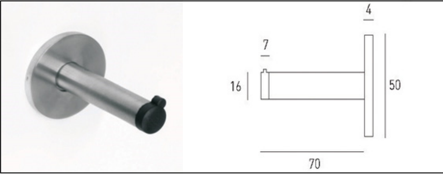
QT - 108 Hook / door stopper concealed fixing made in Stainless Steel AISI 304.
